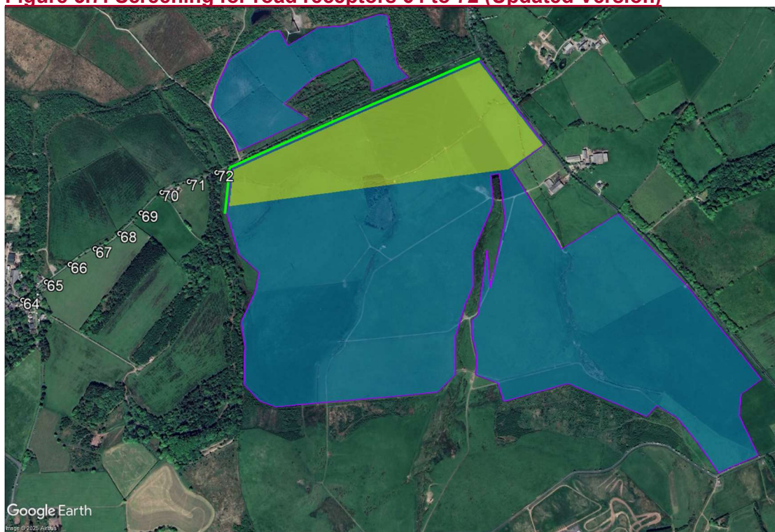
Figure 5.7: Screening for road receptors 64 to 72 (Updated Version)
