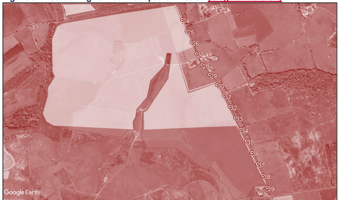
Figure 5.4: Screening for road receptors 24 to 39 (Original Version)
